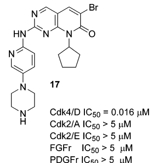
Figure 4. A potent and selective Cdk4 inhibitor.
