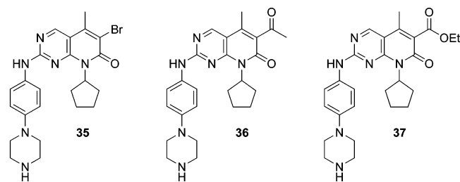
Figure 5. Selective Cdk4 inhibitors containing aniline side chains.
