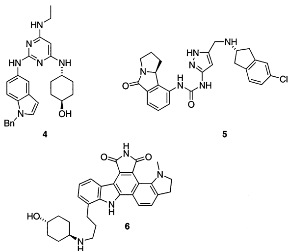
Figure 2. Selective Cdk4 inhibitors.
